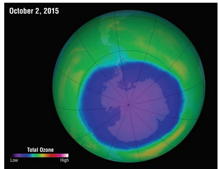
● FIGURE 1.7 The darkest color represents the area of lowest ozone concentration, or ozone hole, over the Southern Hemisphere on October 2, 2015. Notice that the hole is larger than the continent of Antarctica. A Dobson unit (DU) is the physical thickness of the ozone layer if it were brought to Earth's surface, where 500 DU equals 5 millimeters.
