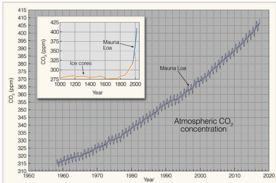
● FIGURE 1.6 (a) The solid blue line shows the average yearly measurements of \text{CO}_2 in parts per million (ppm) at Mauna Loa Observatory, Hawaii, from 1958 to mid-2017. The jagged dark line illustrates how higher readings occur in winter where plants die and release \text{CO}_2 to the atmosphere, and how lower readings occur in summer when more abundant vegetation absorbs \text{CO}_2 from the atmosphere. (b) The inset shows \text{CO}_2 values in ppm during the past 1000 years from ice cores in Antarctica (orange line) and from Mauna Loa Observatory (blue line). (Mauna Loa data courtesy of NOAA; Ice Core data courtesy of Carbon Dioxide Information Analysis Center, Oak Ridge National Laboratory)
